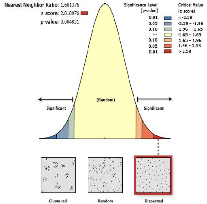
Given the z-score of 2.81807577698, there is a less than 1% likelihood that this dispersed pattern could be the result of random chance.
