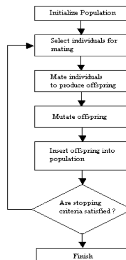
Fig. 2. Genetic algorithm flowchart
