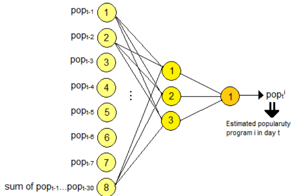
Fig 4: Structure of proposed neural network
