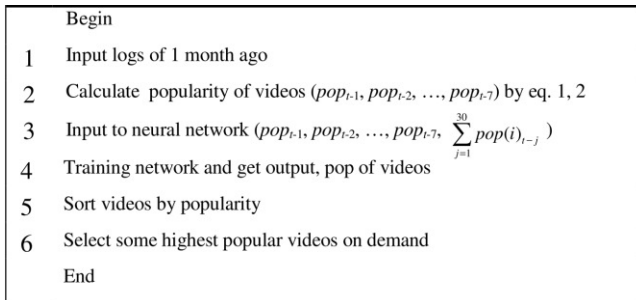
Fig 5: Pseudo code of proposed algorithm
