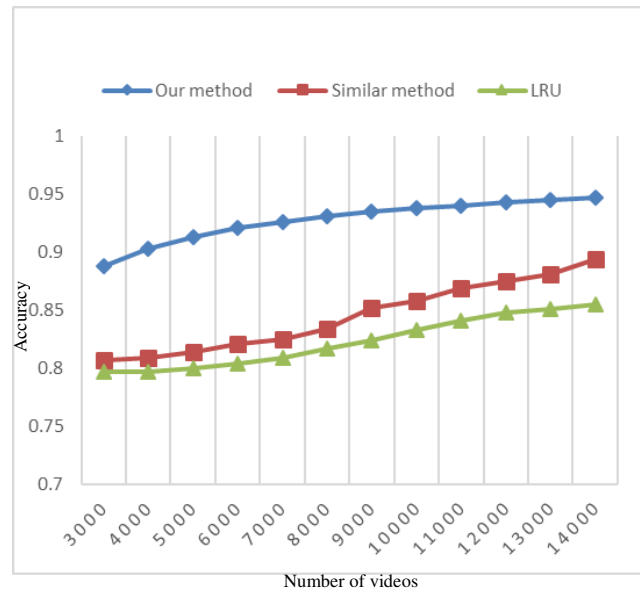
Fig 6: Accuracy curves of different algorithms
