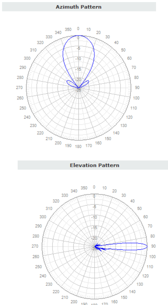
Figure 7. Radiation pattern DualPol .Antenna
