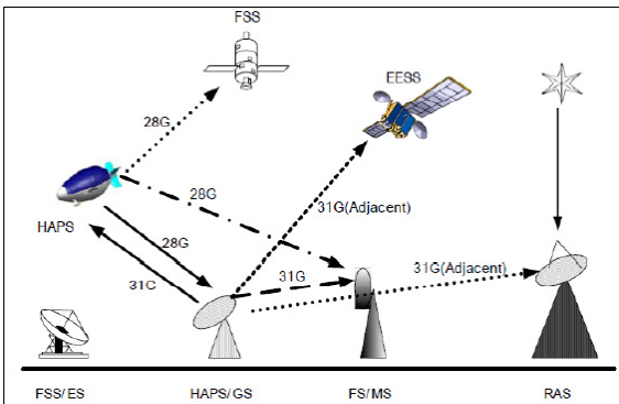
Figure 2. Interference from HAPS into other Communication systems with frequency used
