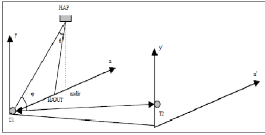
Figure 3. Geometry of interference between HAP and TML
