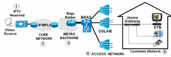
Fig 2: Structure of an IPTV System
