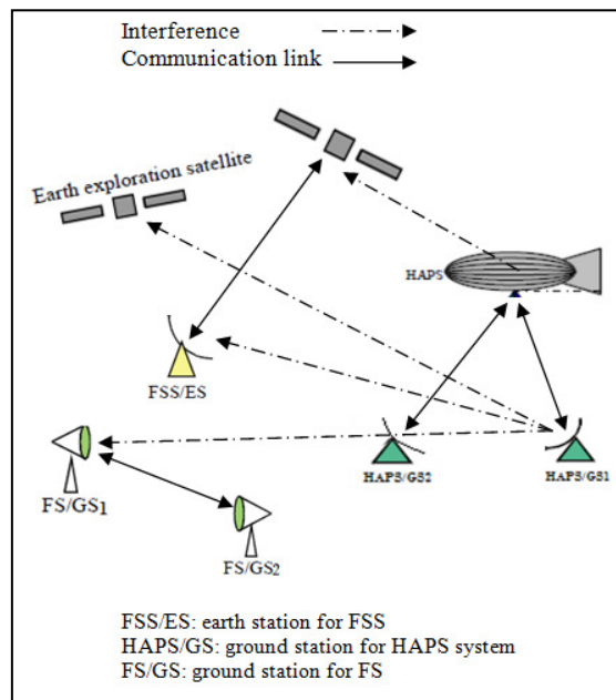
Figure 5. Scenario of Interference situation including HAPS, FSS, FS.
