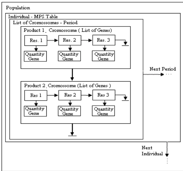
Fig. 2. Chromosome representation
