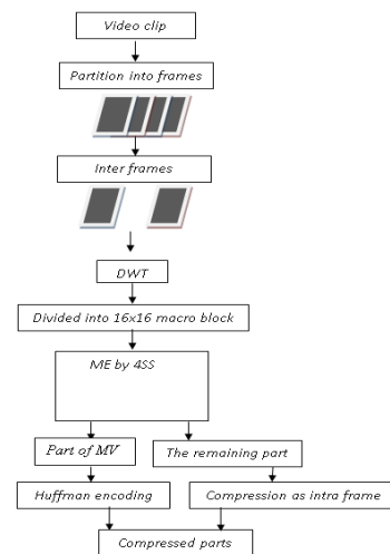
(a): Compression stage Fig. 4: The flowchart of inter coded frames with in clip.
