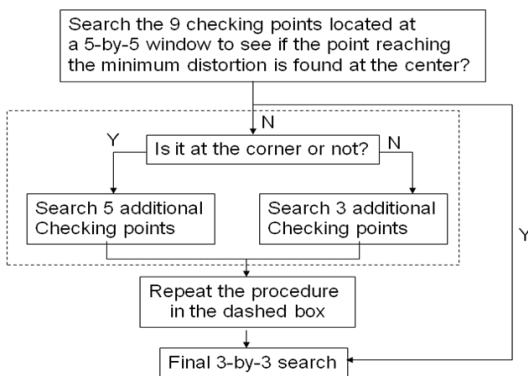
Fig. 2: Flow chart of 4-step search
