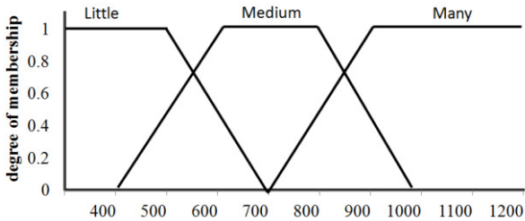
Figure (4) Membership functions for Salary
