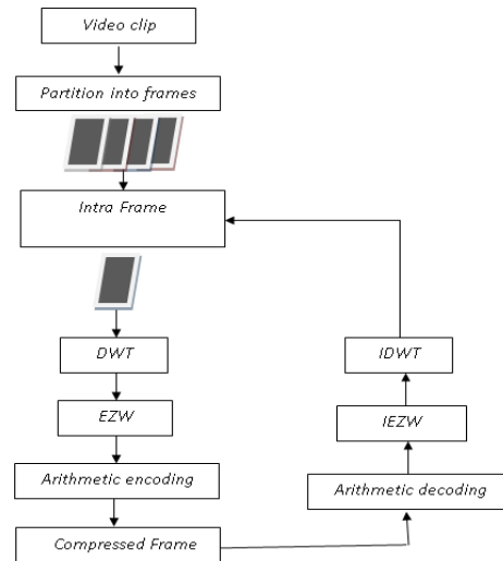
Fig. 3: The flowchart of intra coded frame of clip
