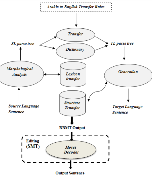
Fig. 2. Architecture of Arabic-English HMT System
